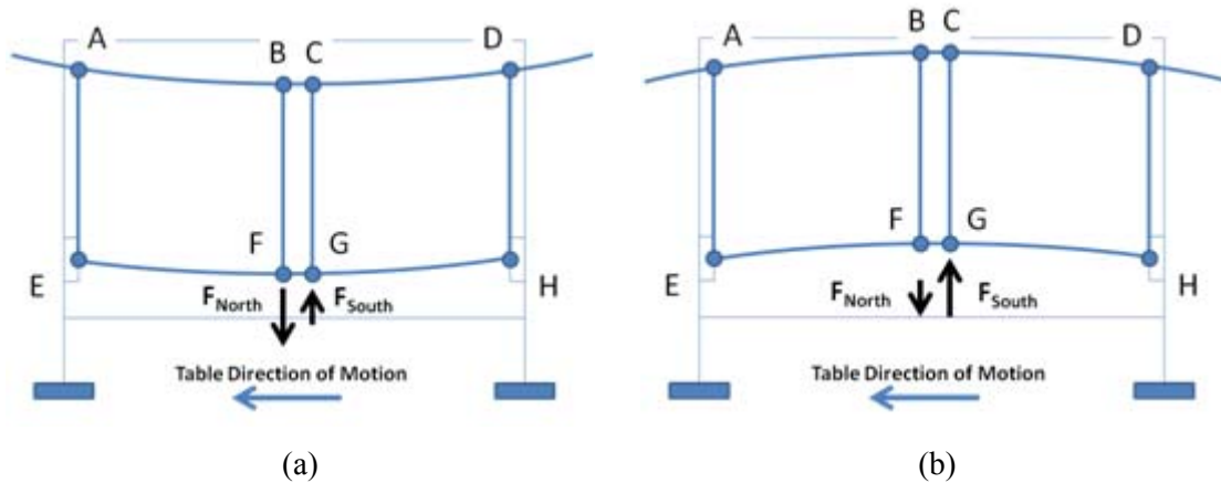
Figure 3.12 Unequal load distribution when table is moving in positive direction. (a) North panel with larger force contribution. (b) South panel with larger force contribution.
