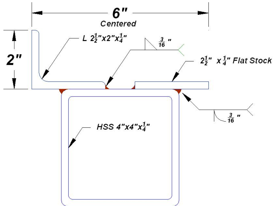
Figure 3.13 Detail of section I for members A-D and E-H
