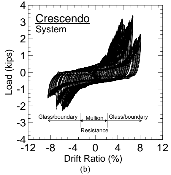
Figure 3.6 Global response from tests (a) Monotonic 4 and (b) Crescendo 3 –Two-5'x5' specimens with 2mil of film unattached.
