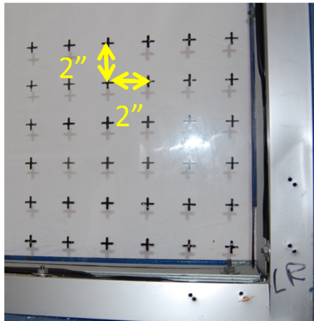
Figure 2.27 Two inch square grid pattern spray painted into each corner of the glass to aid damage tracking
